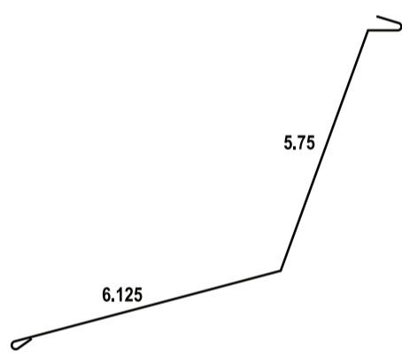
13. CHIMNEY FLASHING
