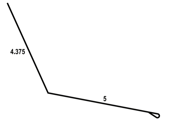
8. ENDWALL FLASHING
