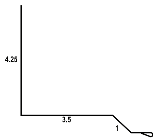
9. SIDEWALL FLASHING
